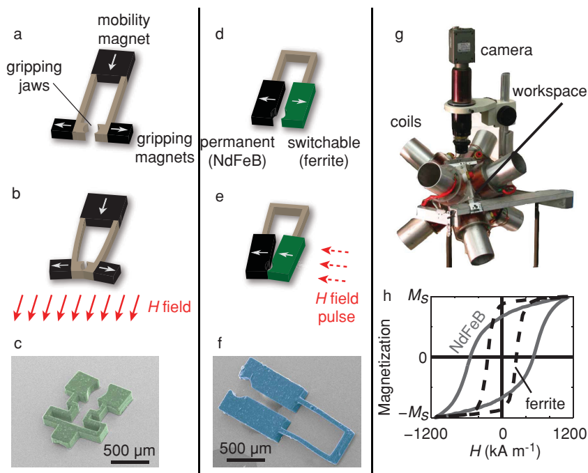
Figure 1. Remotely-actuated untethered micro-gripper designs. a–c) Torque-based addressable micro-gripper. This micro-gripper is closed by application of a constant uniform magnetic field, which exerts a torque on each gripper arm. The “mobility magnet” acts to move the gripper as a mobile robotic device. c) A scanning electron microscope (SEM) image of a fabricated torque-based gripper. d–f) Force-based addressable micro-gripper. The gripping state is changed through the application of a large magnetic field pulse, which switches the ferrite magnet magnetization directions. This changes the arms from a repulsive to attractive state. The micro-gripper can be re-opened by applying a field pulse in the opposite direction. f) An SEM image of a fabricated force-based gripper. g) Magnetic coil system used to apply low and moderate fields of up to 22 kA m -1 . h) Magnetization hysteresis loops of NdFeB and ferrite magnetic materials used, as measured in an alternating force gradient magnetometer. This shows the magnetization of the permanent material NdFeB and the switchable material ferrite as a function of applied field H . Each curve is normalized to the saturation magnetization M_s of the material.
