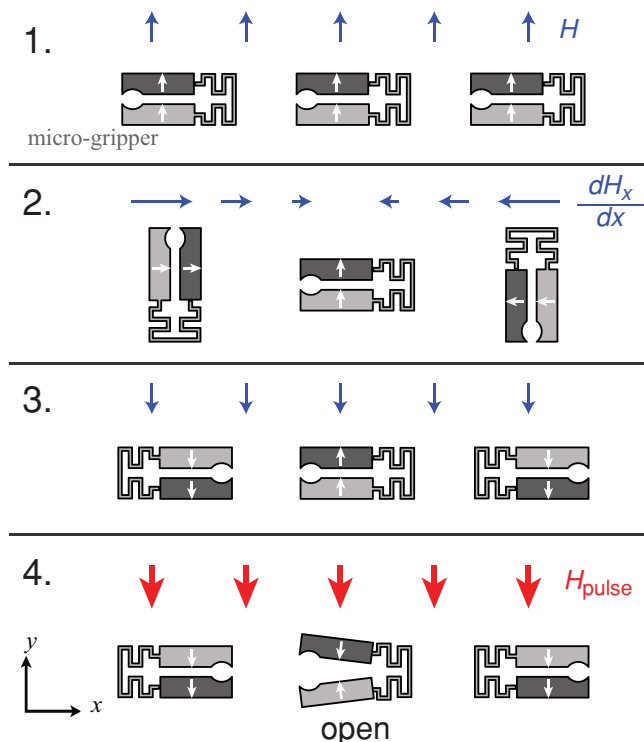
Figure 4. Selective orientation process to achieve addressable opening and closing of individual micro-grippers among a set. Gripper tip magnetization is shown as arrows. Dark sections indicate permanent NdFeB magnet materials, while light sections indicate switchable ferrite material.
