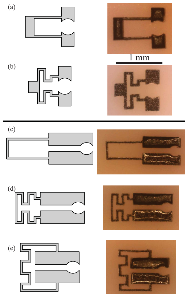
Figure 3. Fabricated micro-gripper shapes. Micro-gripper designs, with CAD model on the left and fabricated polymer-based flexible designs on the right. a,b) Torque-based designs, showing simple and meander flexure design. Each design has approximately the same flexure stiffness. The mobility magnet is seen on the left side of the design. (c–e) Force-based designs, showing simple and meander flexure design.
