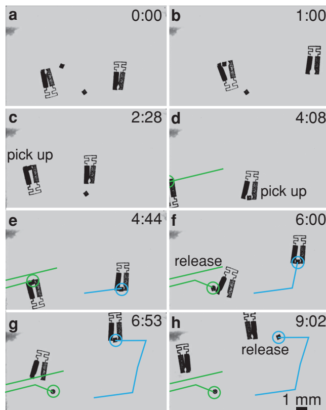
Figure 6. Parallel operation of two addressable mobile micro-grippers. a) Two identical micro-grippers start in the closed configuration, with two polyurethane disks nearby. b) The first micro-gripper approaches a disk. c) The first gripper is closed over the disk, grasping it. d) The second micro-gripper is positioned over the second disk, while the first gripper retains its cargo. e) Both micro-grippers have grasped their cargo and carry it in parallel to the desired location. f) The first gripper releases its cargo. g) The second gripper moves to its goal position. h) The second gripper releases its cargo. Time indicated on each pane is minutes:seconds. A video of assembly and actuation are shown in Supporting Information Video 3.
